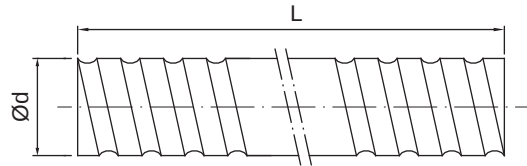
Fig 2.3.1 Screw Shaft Nominal Diameter
