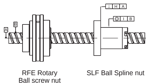
Fig 1.2.2 NSH - series
