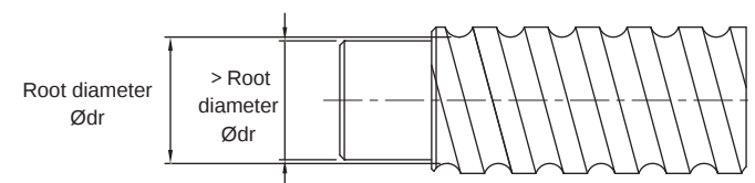
Fig 1.10.4 For Internal Circulation
