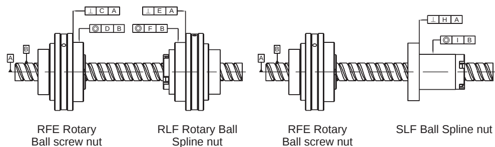
Fig 1.2.1 NSV - series
